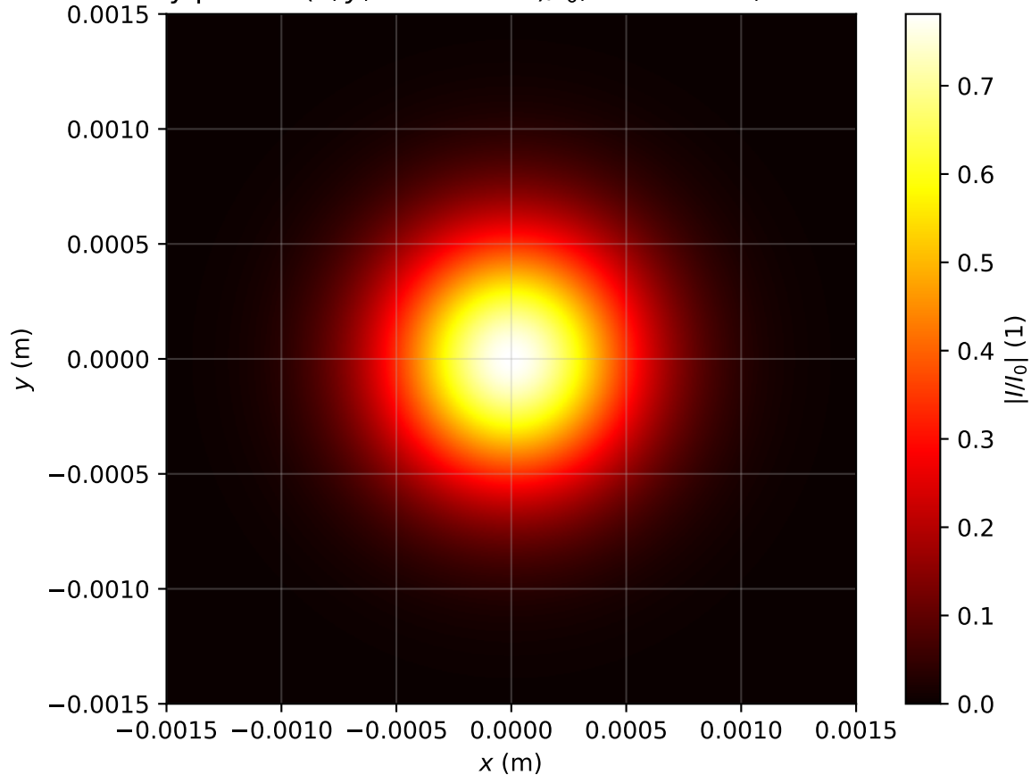
Intensity profile I(x, y, z = 1.353m)/I_0 , P_{in}=0.2P_{cr} , artificial time
